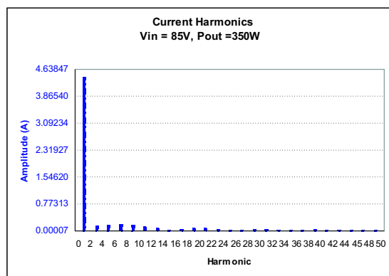
Figure 7. Current Harmonics
