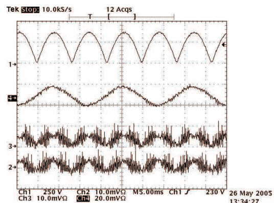
Figure 12. V_{IN} = 265 \text{ V RMS} , P_{OUT} = 350 \text{ W}
